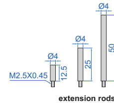
extension rods
